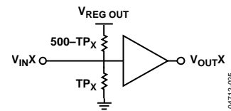
Figure 25. Gamma Buffers Tap Point Circuit.
